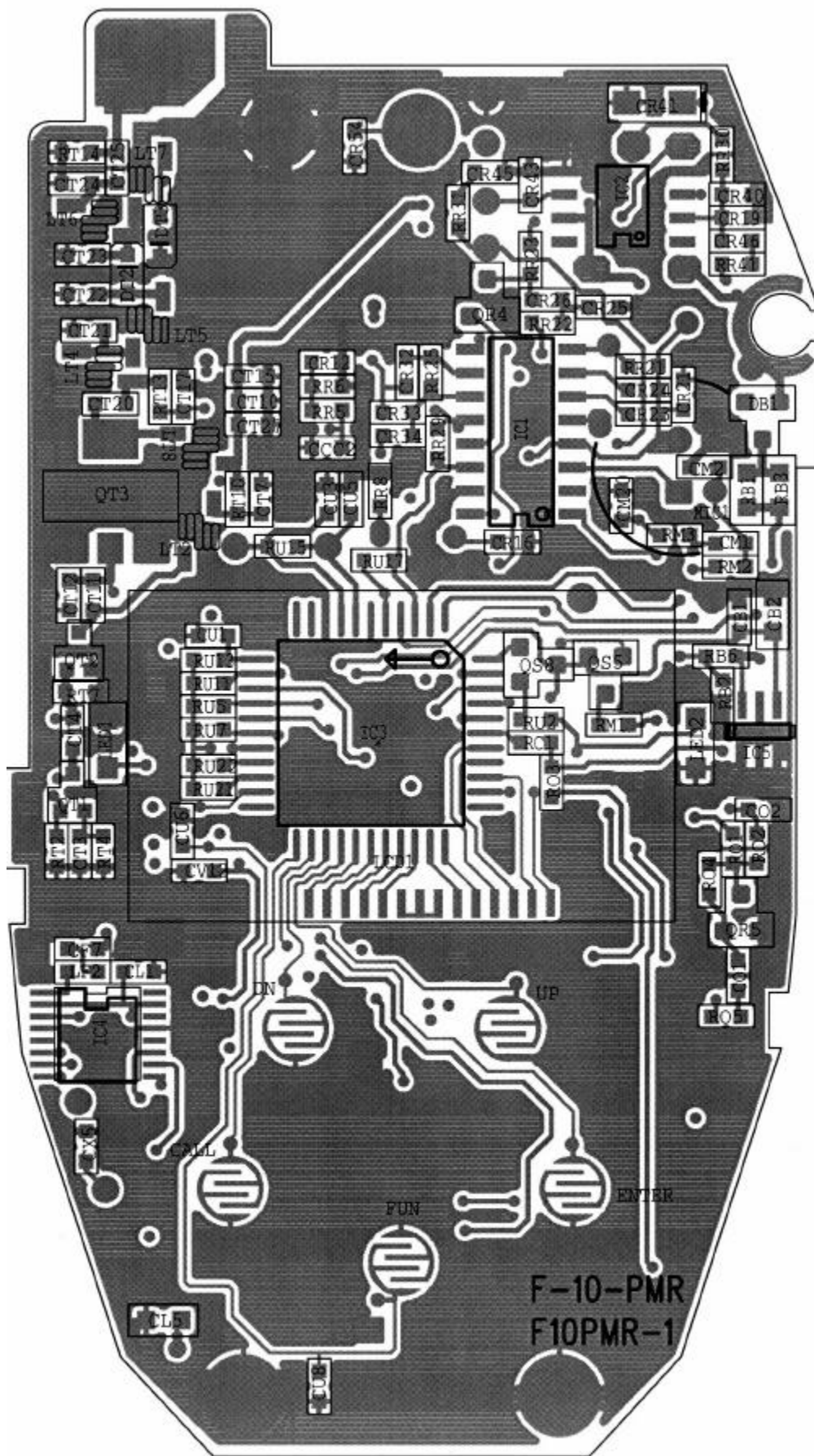
TOP SILK
