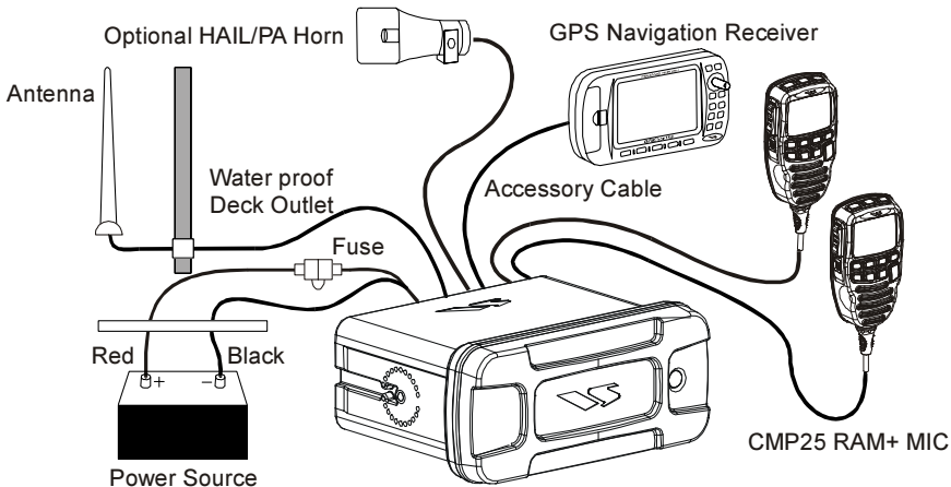
Figure 1. General Installation
