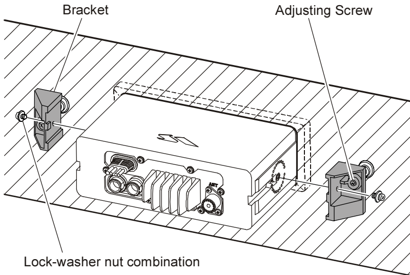
Figure 4. MMB-84 Flush Mount Installation
