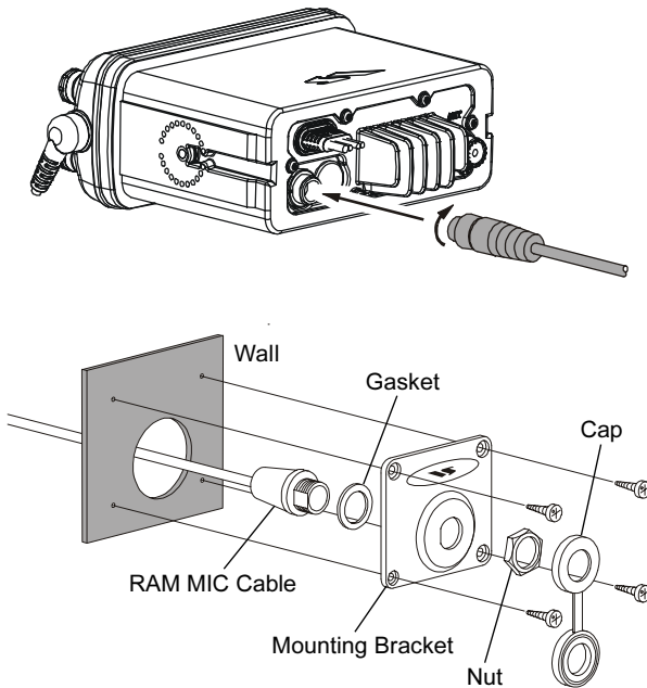
Figure 3. CMP25 RAM+ MIC Installation
